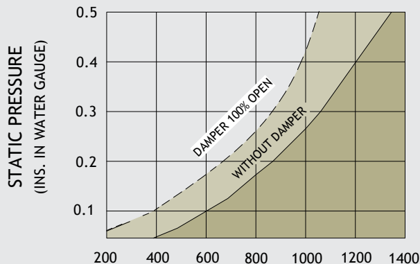
VOLUME OF AIR FLOW (C.F.M.)
